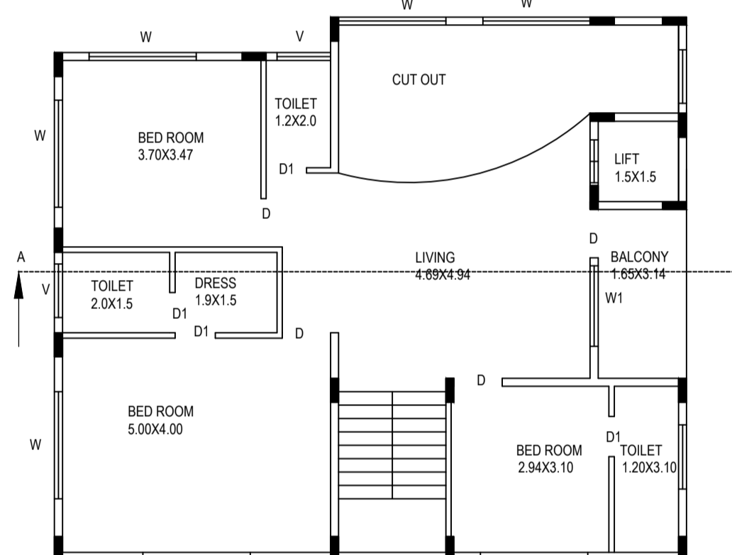
TYPICAL FIRST AND SECOND FLOOR PLAN
